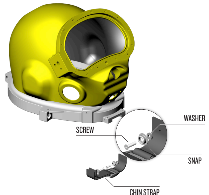
The chin strap mounts inside the helmet.
