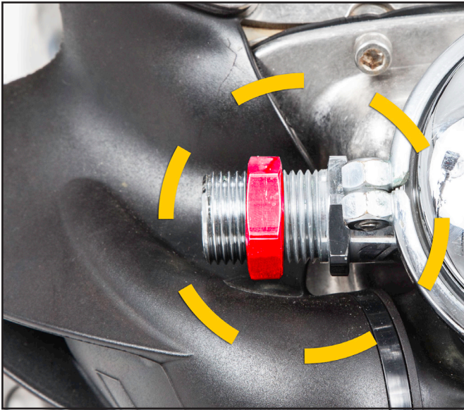
INCORRECT Jam Nut position prior to attaching the Bent Tube Assembly.
