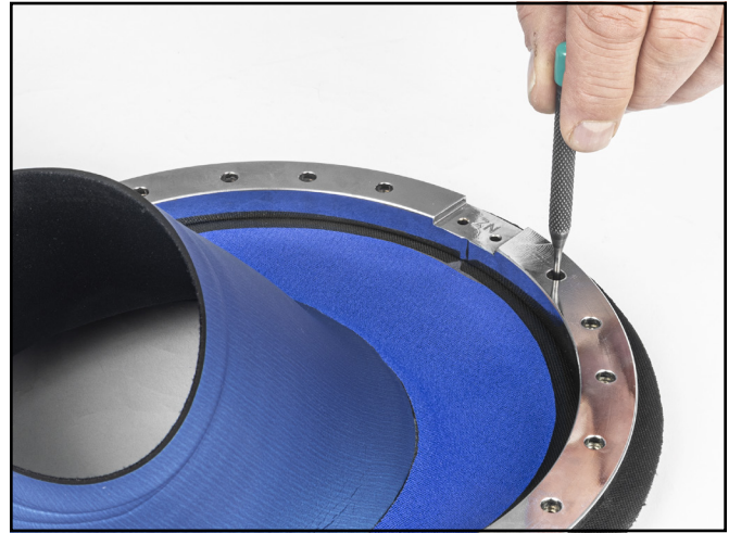
Use a small, sharp punch to locate the bottom hole.
