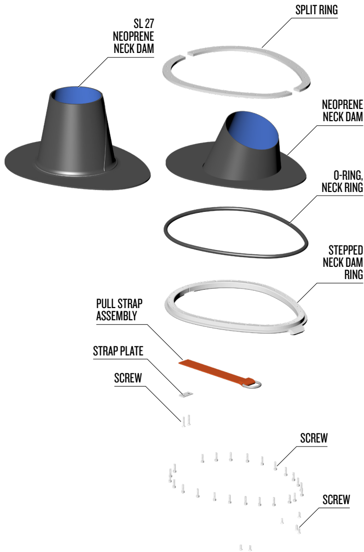
Neck ring assembly for the helmet.
