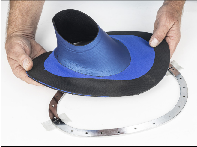
Place the neck dam on top of the split rings.
