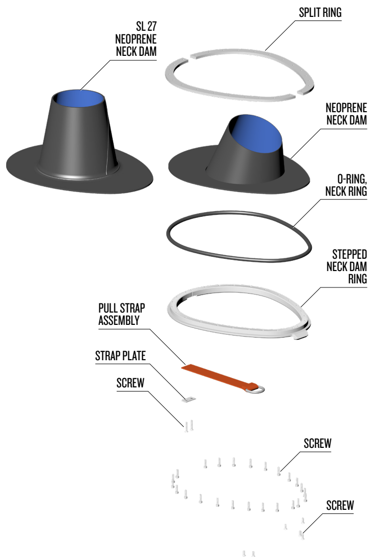
Neck ring components.
