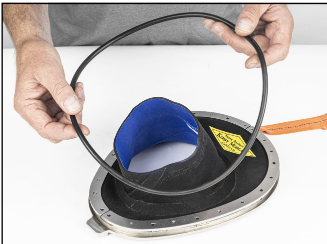
Inspect the O-ring on the neck ring.
