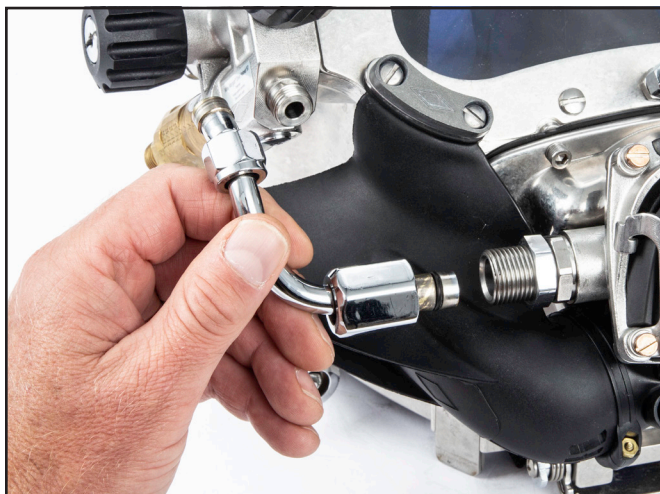
Install the bent tube assembly.
