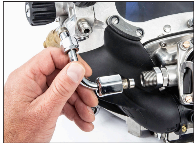
Remove the bent tube assembly.
