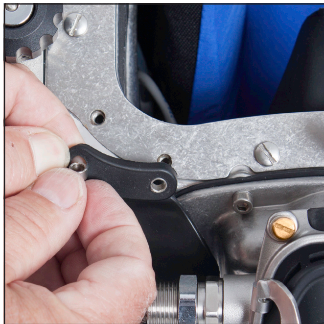
Attach the whisker to each side of the face port retainer using the spacers, zinc anodes or kidney plates and screws.
