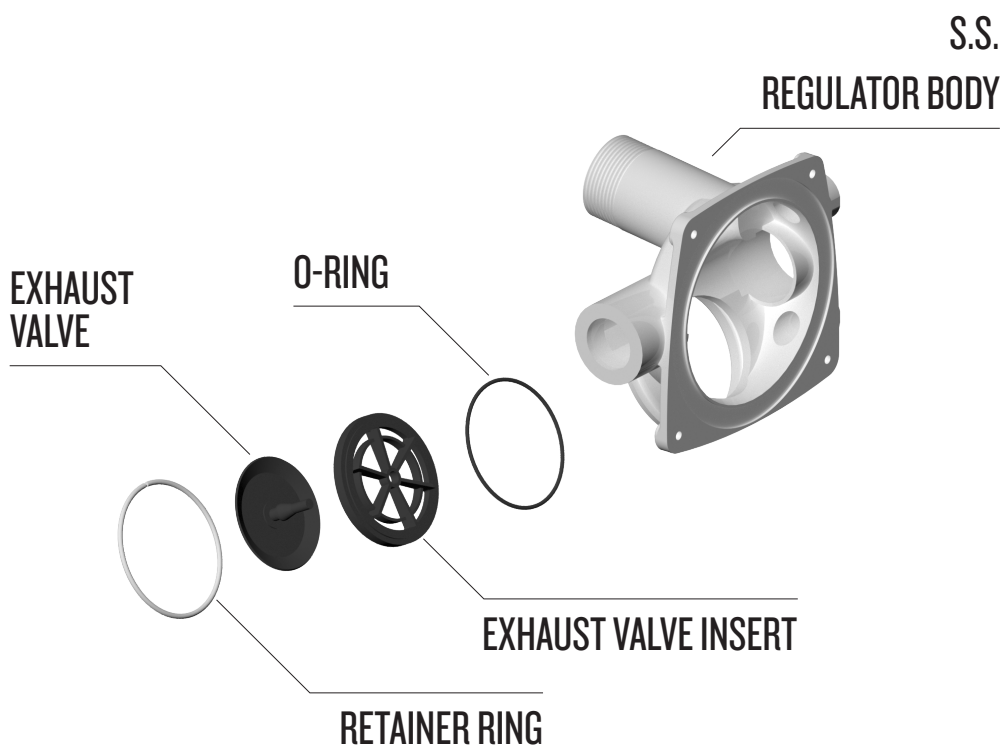
455 Balanced exhaust valve mechanism.
