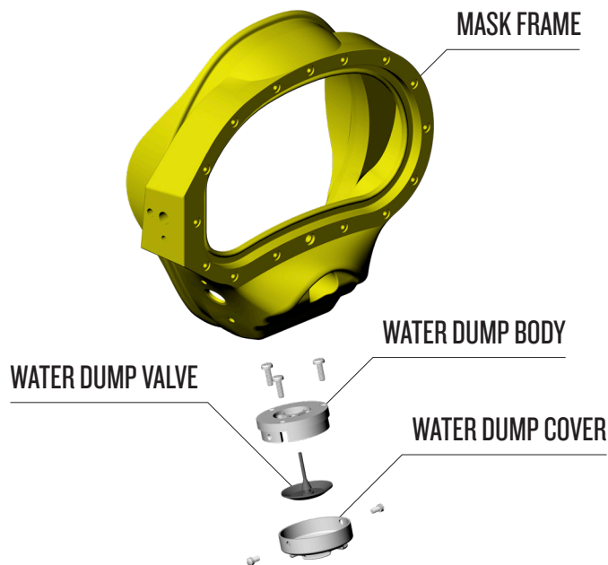
28 Water Dump Cover P/N 545-041
